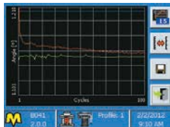
Test data plot
