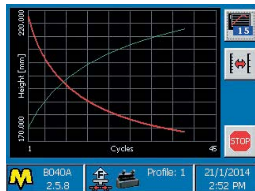
Height-Cycles and Density-Cycles curves during compaction
