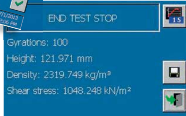
End test data (with shear stress value)
