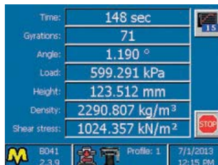
Test execution with shear stress measurement
